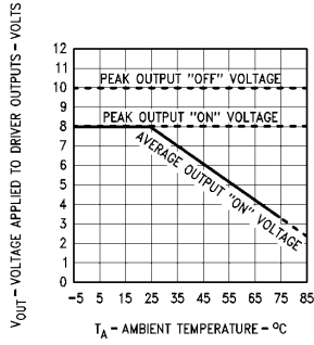
FIGURE A. Output Voltage Safe Operating Area
