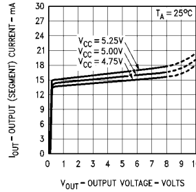
FIGURE B. Typical Constant Segment Current Versus Output Voltage
