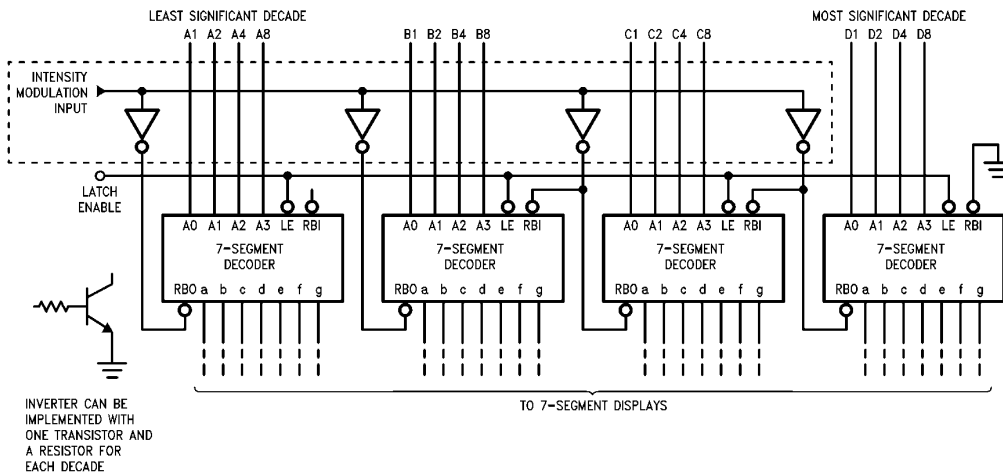
FIGURE D. Intensity Control by \overline{RBO} Pulse Duty Cycle
